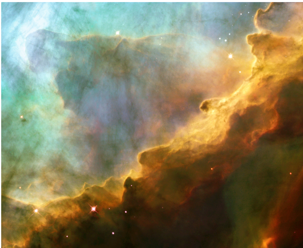
Omega Nebula
